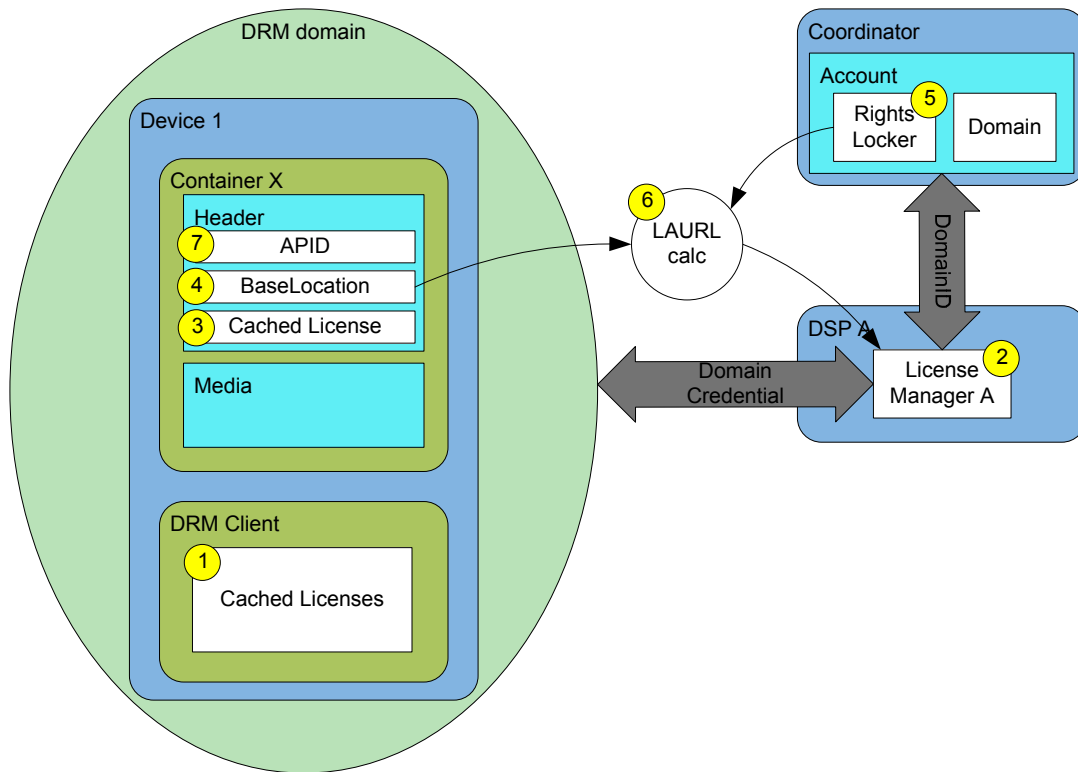
Figure 17 – License Acquisition (simplified) (informative)
