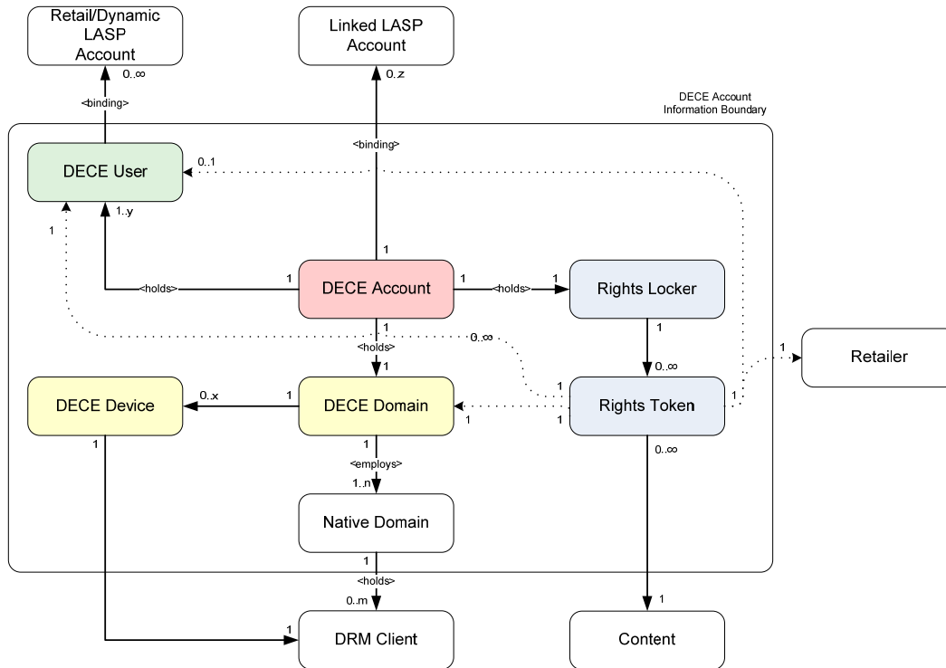
Figure 1 – Entity – Relationship Diagram (Informative)
